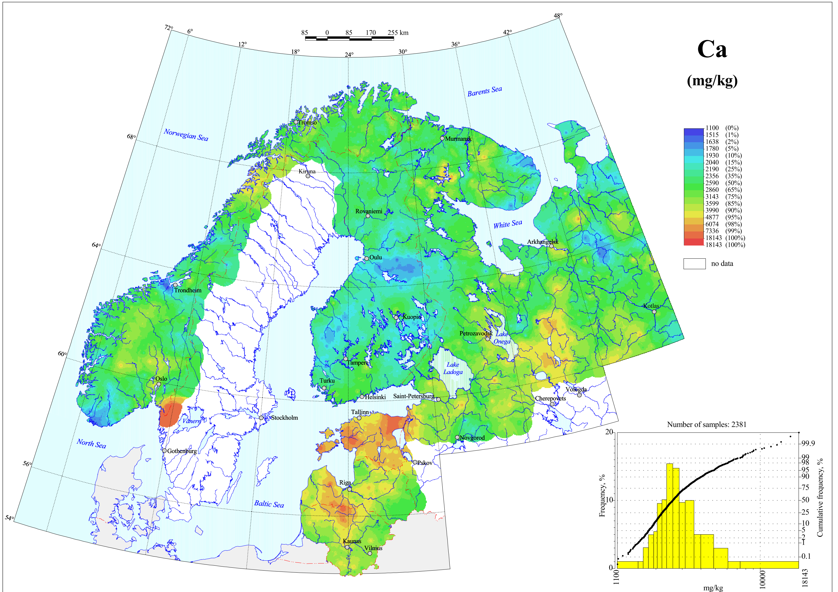
Calcium in Terrestrial Moss, Total Content
